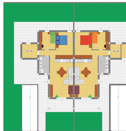
Planimetria Piano terra
